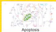
Apoptosis
